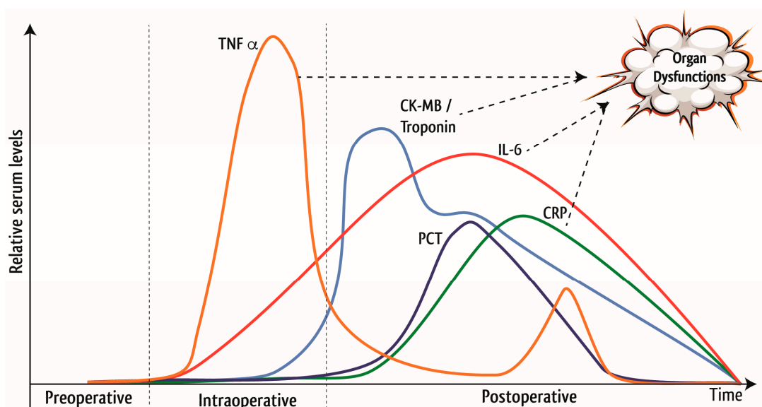
Figure 1. Time course of inflammation and development of organ dysfunction in cardiac surgery. Cardiac surgery leads to an anticipated rise of inflammatory mediators, such as TNF \alpha , IL-6, procalcitonin (PCT), c-reactive protein (CRP) and markers of myocardial damage, such as creatine kinase (muscle/brain) (CK-MB) and troponin [11]. These mediators trigger the development of postoperative organ injuries, which are explained in greater detail in Figure 2.
